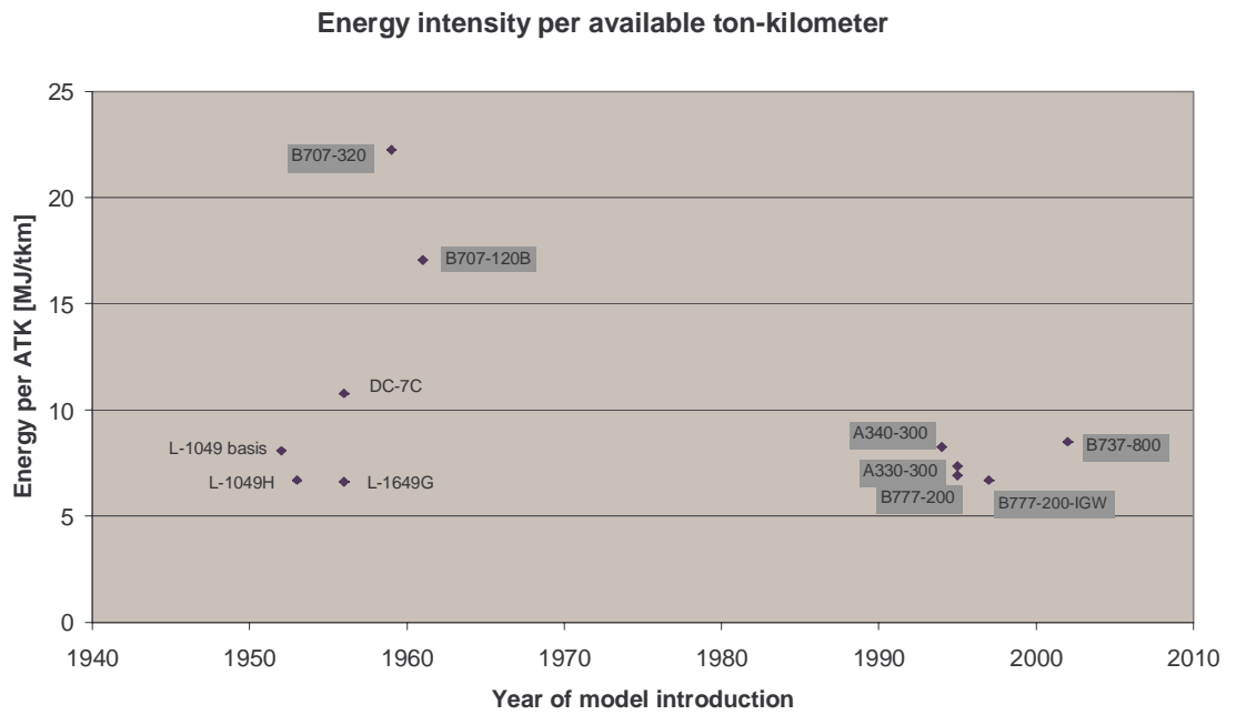
Figure 6: Energy intensity per available ton-kilometre.
