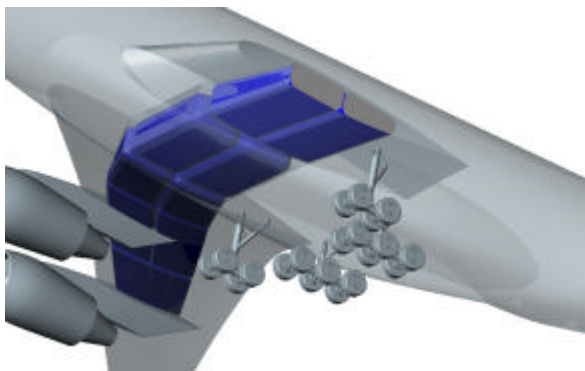
Figure 18: Modified A380 for short range operation
